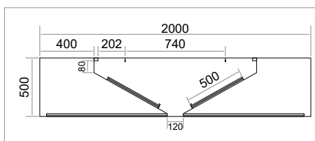
TYPE HCL 2000
