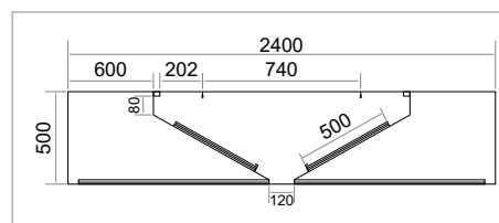
TYPE HCL 2400
