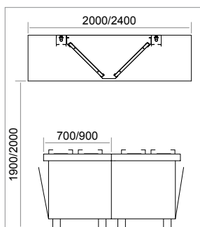
TYPE HCL 2000
