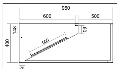
TYPE HRL 400x950
