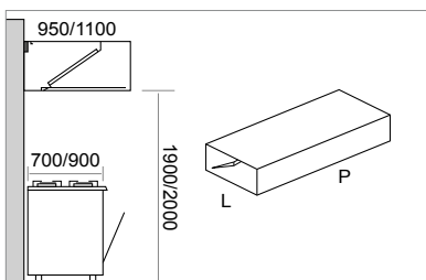
TYPE HRL 540x950
