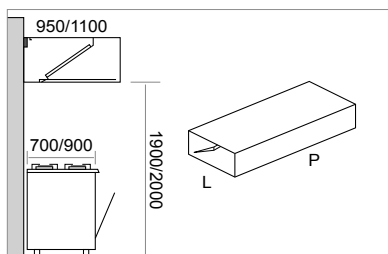
TYPE HRL 400x950
