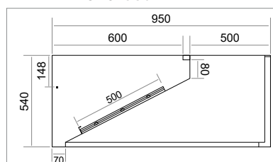
TYPE HRL 540x950
